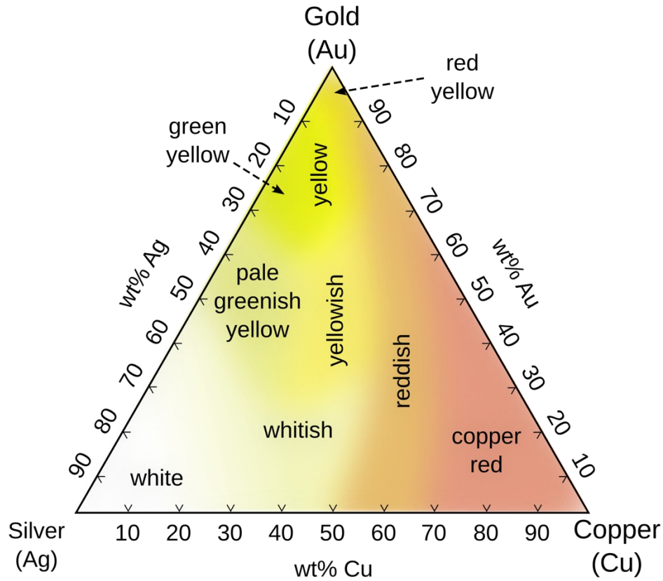
Figure 17. A ternary plot illustrating colors of gold alloys determined by concentrations of gold, silver, and copper. 65
